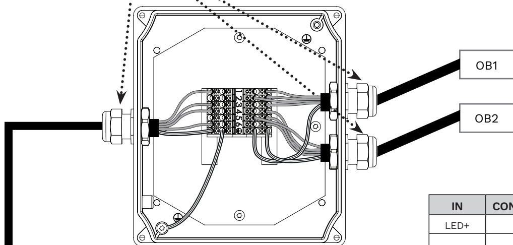
Connections inside Junction box
